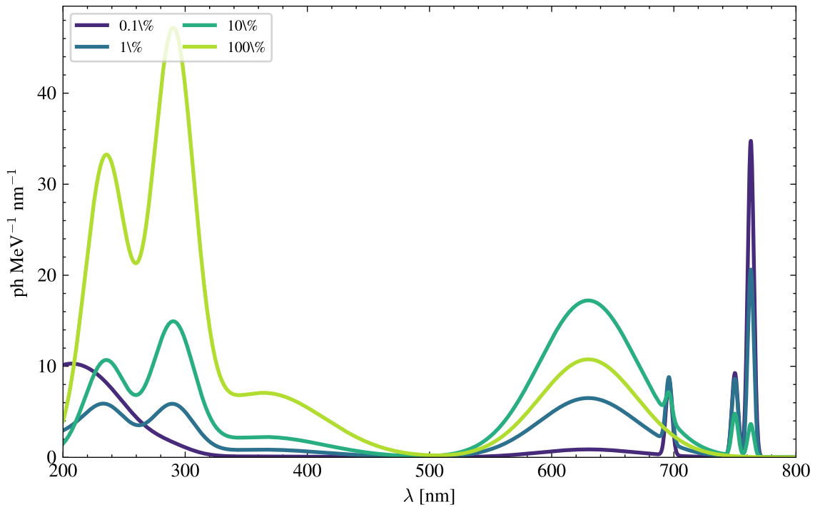
Primary Ar--CF 4 spectra, 2 bar
