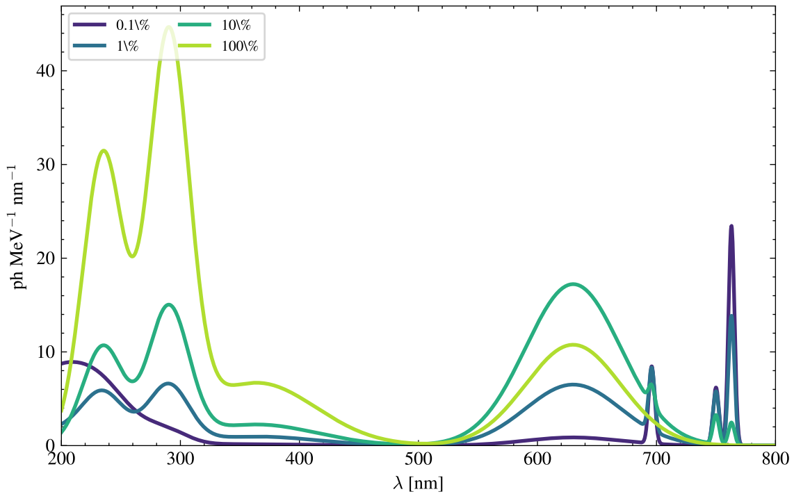
Primary Ar--CF 4 spectra, 3 bar
