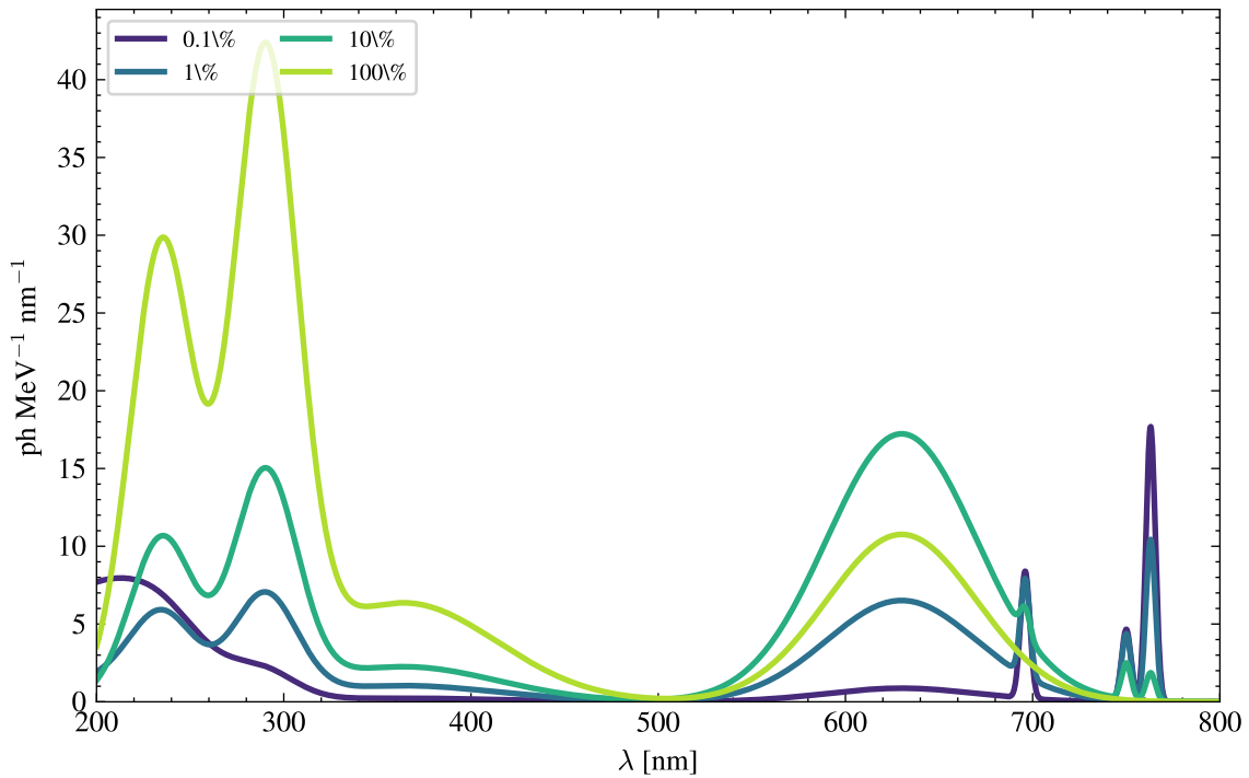
Primary Ar--CF 4 spectra, 4 bar
