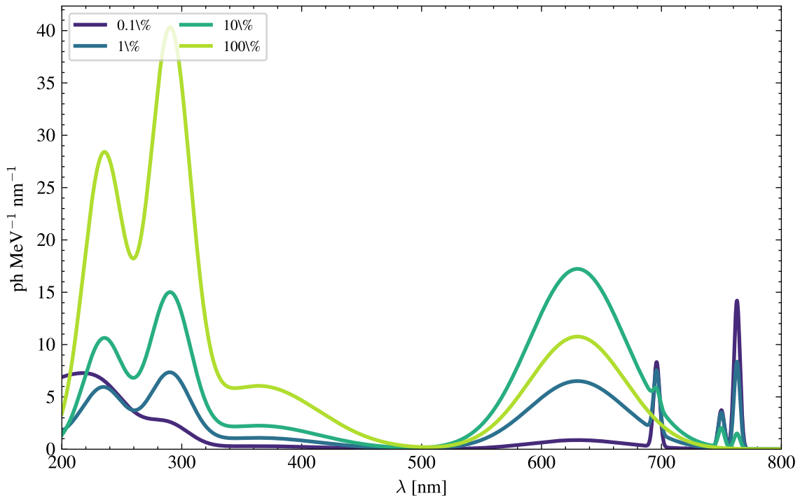
Primary Ar--CF 4 spectra, 5 bar
