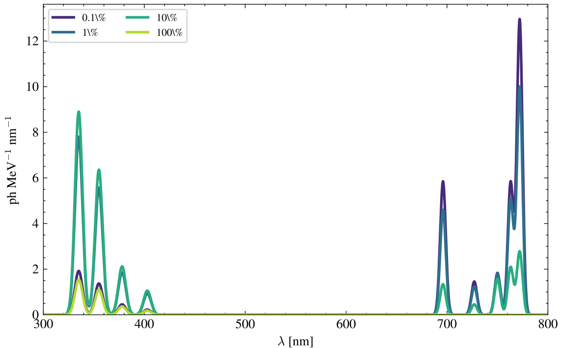
Primary Ar--N 2 spectra, 10 bar
