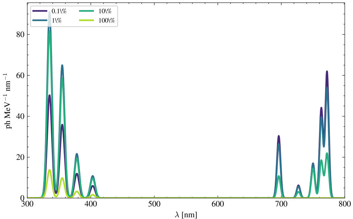
Primary Ar--N 2 spectra, 1 bar
