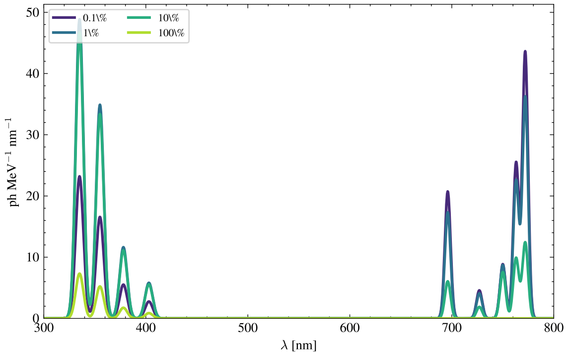
Primary Ar--N 2 spectra, 2 bar
