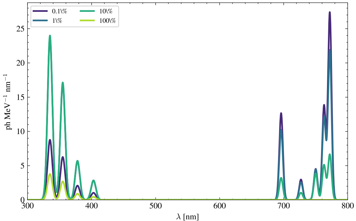
Primary Ar--N 2 spectra, 4 bar
