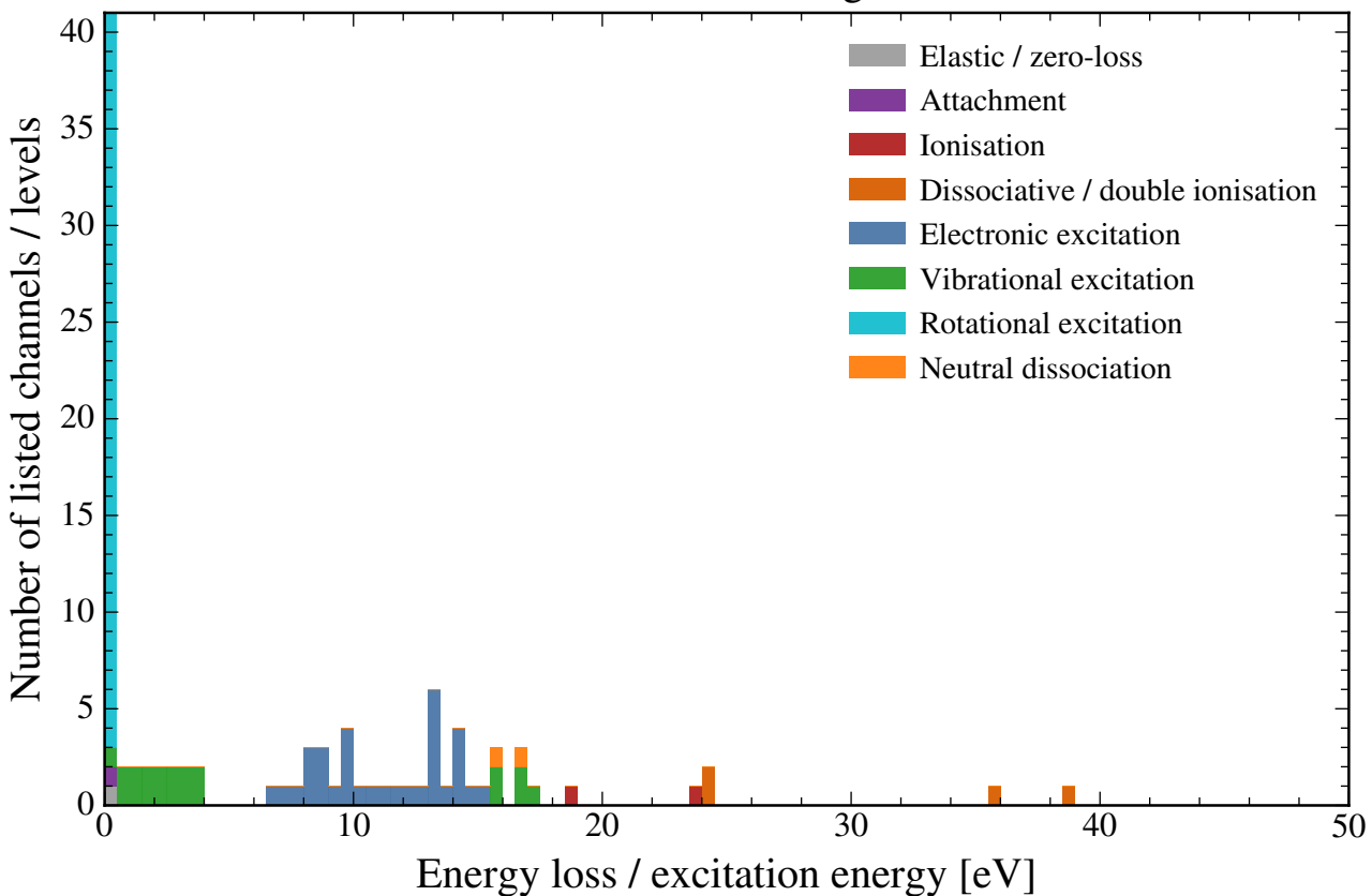
N 2 Garfield++ level catalogue, 0--50 eV
