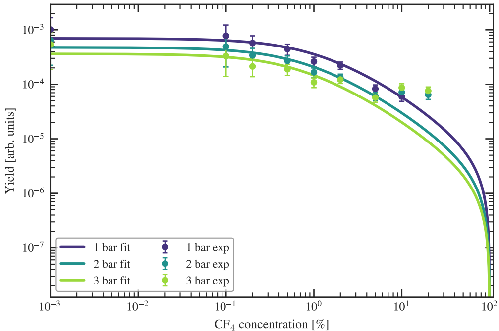
Ar--CF 4 primary IR fit, 696 nm
