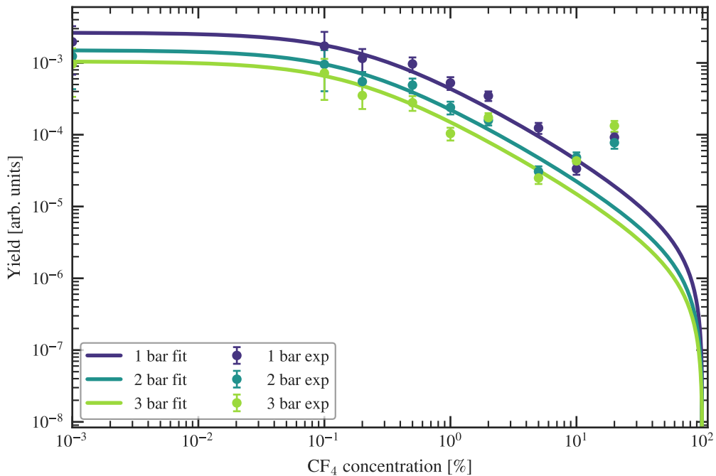
Ar--CF 4 primary IR fit, 772 nm
