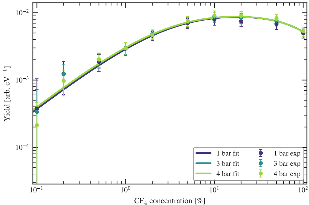
Ar--CF 4 primary visible fit
