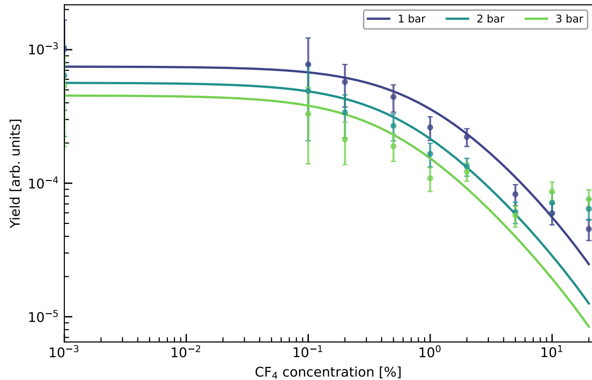
Joint IR fit: ArCF 4 , 696 nm
