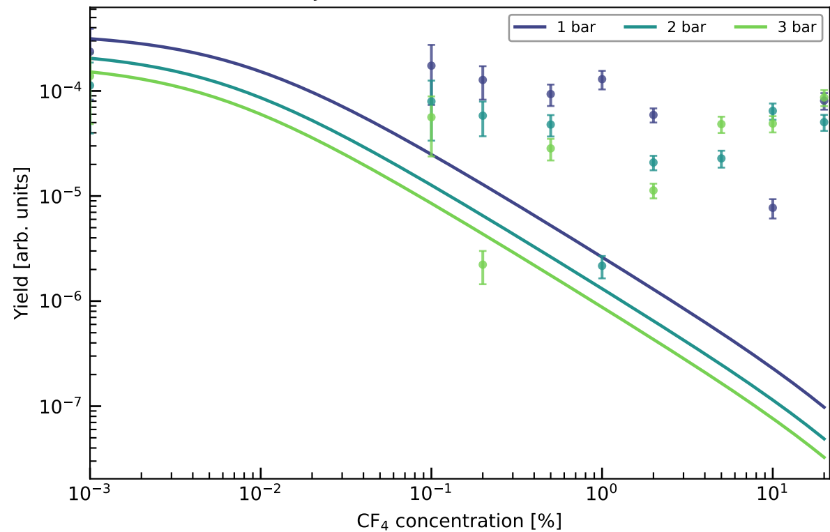
Joint IR fit: ArCF 4 , 727 nm
