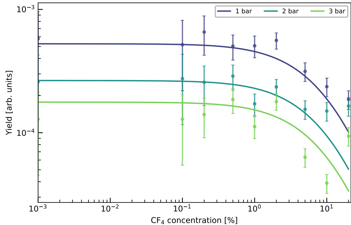
Joint IR fit: ArCF 4 , 750 nm
