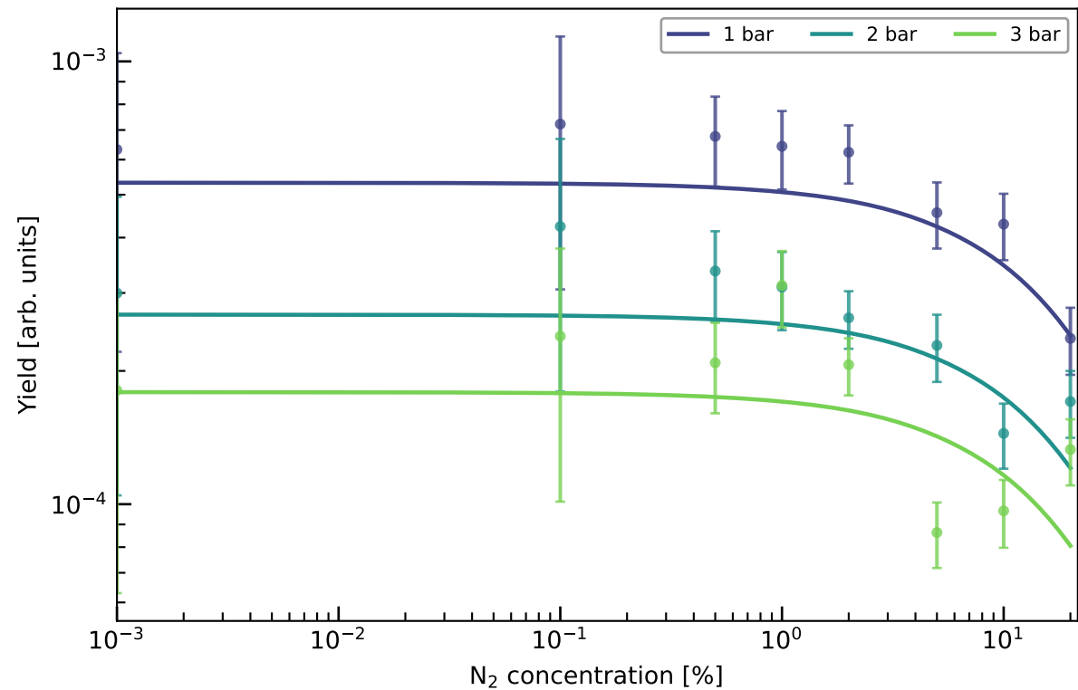
Joint IR fit: ArN 2 , 750 nm
