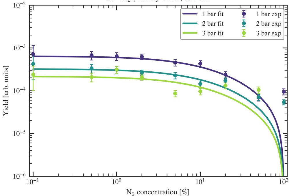
Ar--N 2 primary IR fit, 750 nm
