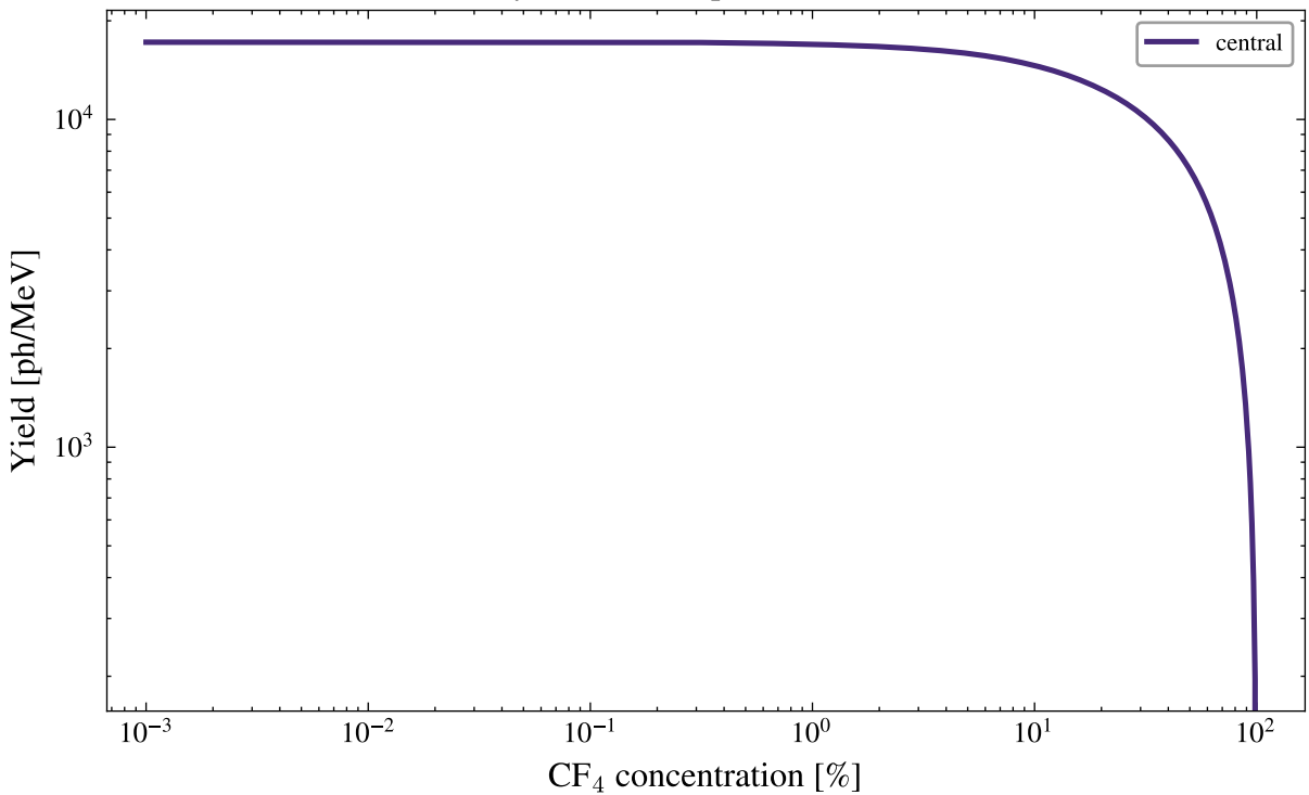
Primary Ar--CF 4 IR prediction, 0.1 mbar
