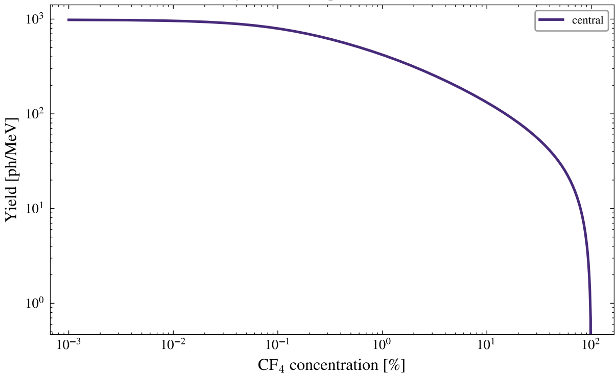
Primary Ar--CF 4 IR prediction, 1000 mbar
