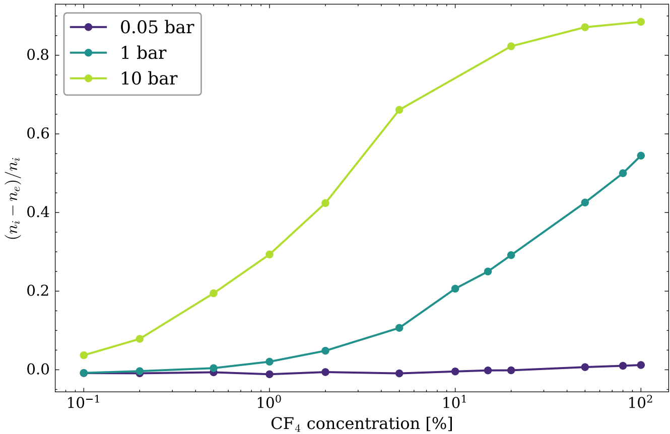
Ar--CF 4 TH-GEM charge balance
