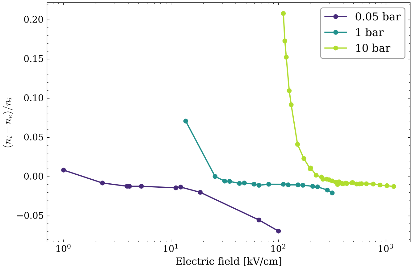
Ar--CF 4 charge balance vs E, 1% CF 4 , N_e = 100 \pm 20
