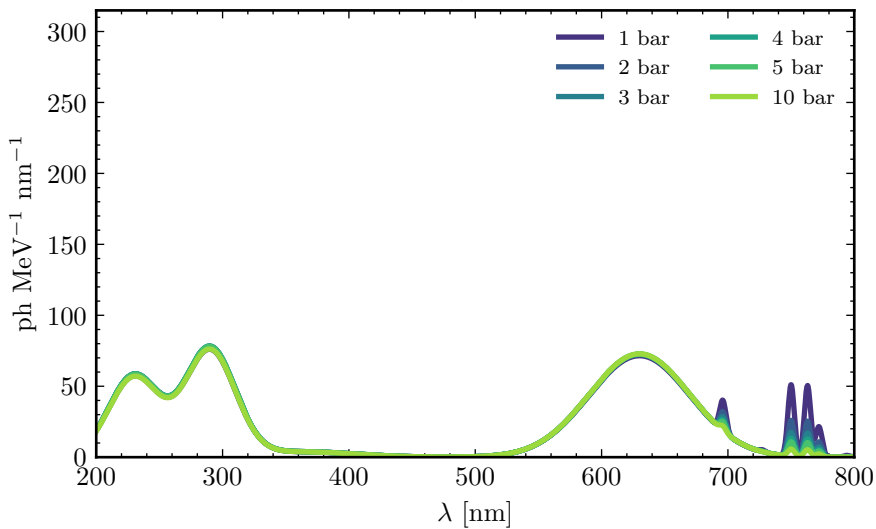
Ar-CF 4 , 10% CF 4
