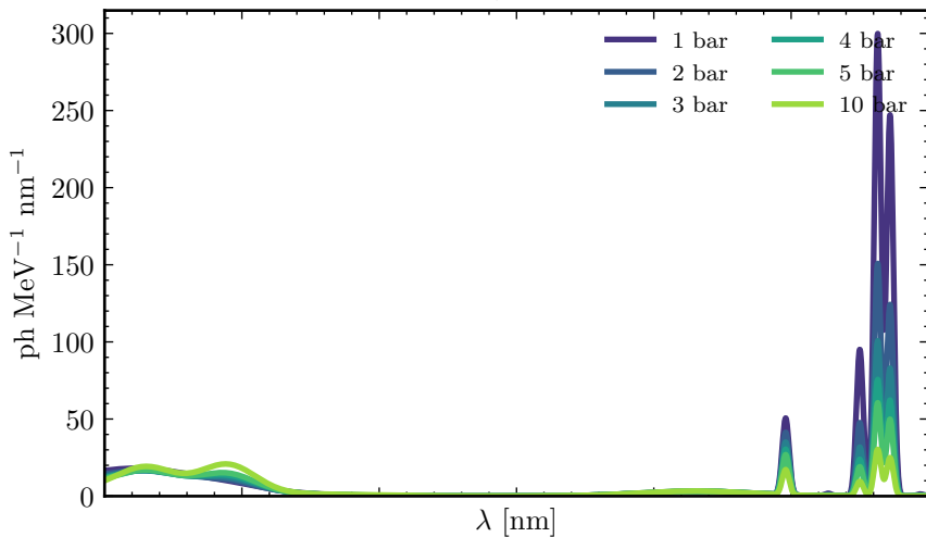
Ar-CF 4 , 10% CF 4
