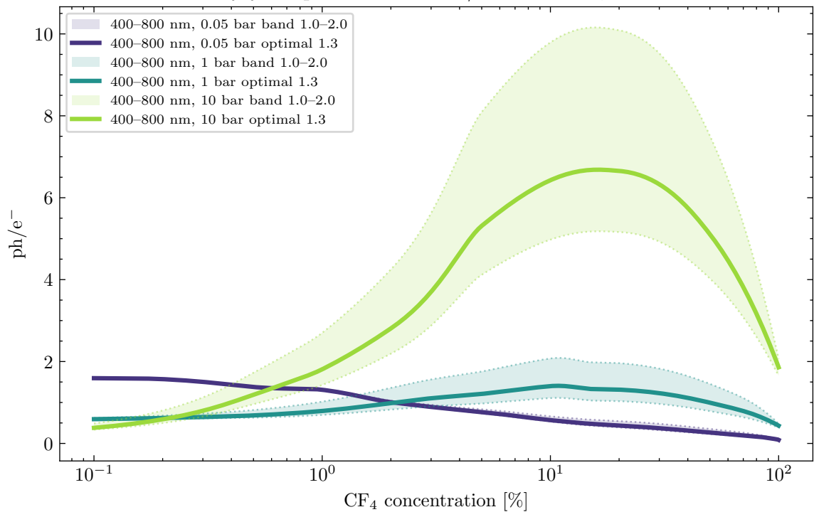
Secondary yield prediction for Ar/CF 4 thGEM, 400–800 nm
