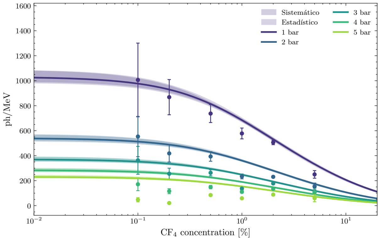
Primary Ar-CF 4 IR yield (680–800 nm)
