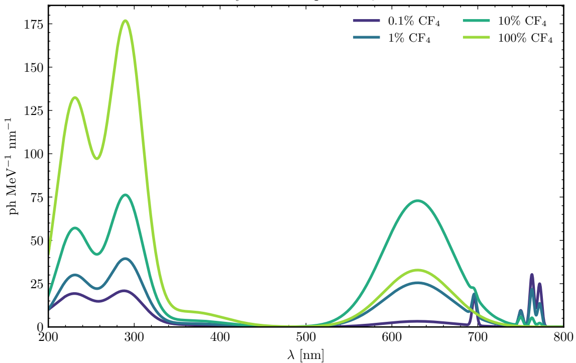
Primary Ar-CF 4 spectrum, 10 bar
