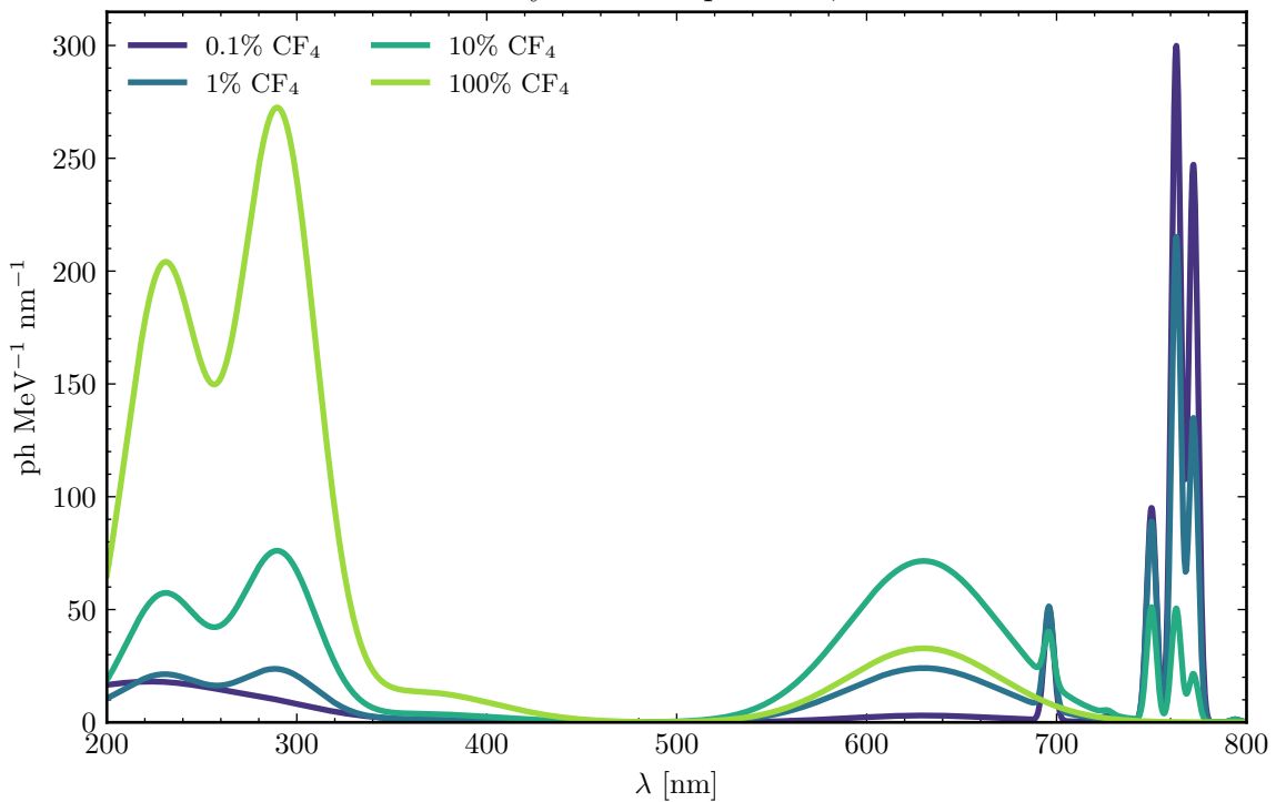
Primary Ar-CF 4 spectrum, 1 bar
