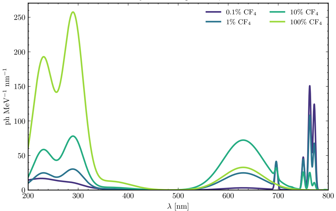
Primary Ar-CF 4 spectrum, 2 bar
