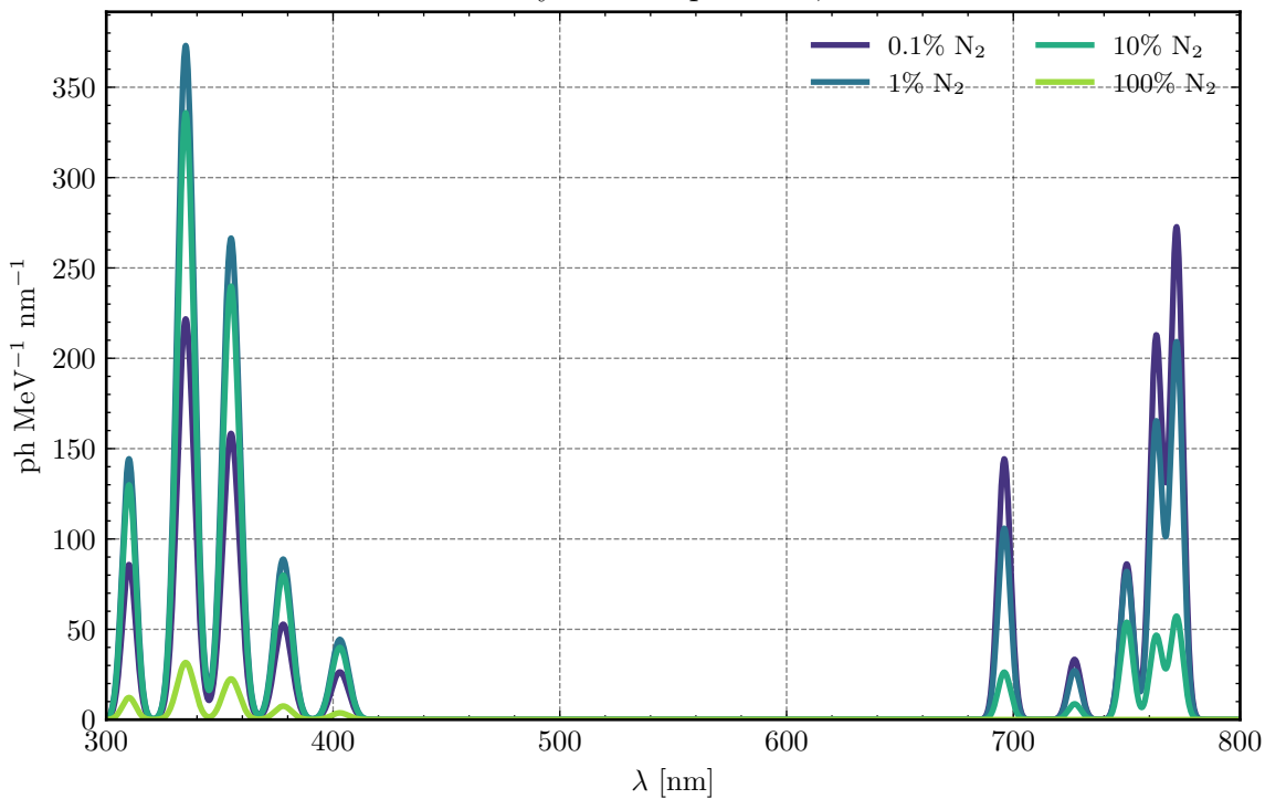
Primary Ar-N 2 spectrum, 1 bar
