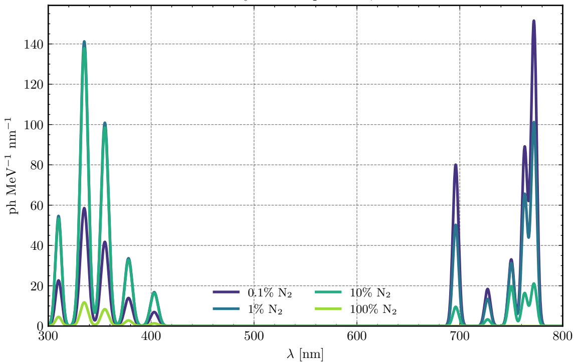
Primary Ar-N 2 spectrum, 3 bar
