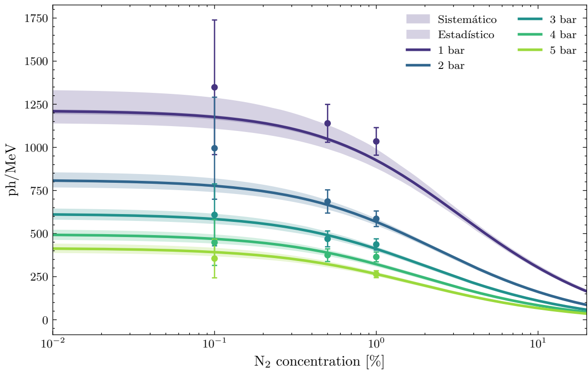
Primary Ar-N 2 IR yield (680–785 nm)
