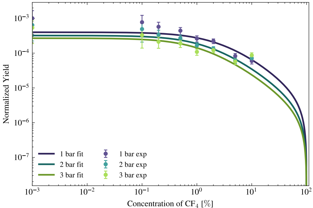
Primary ArCF 4 IR (696 nm) Yield fit
