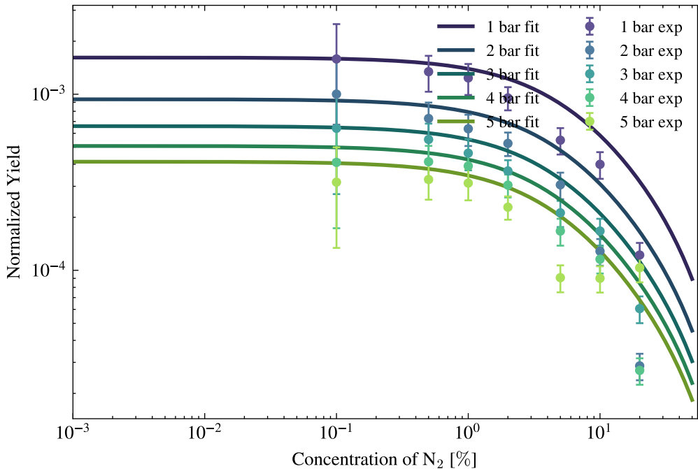
Primary ArN 2 IR (763 nm) Yield fit
