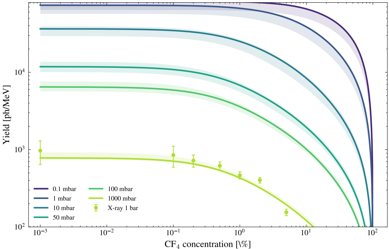
Primary Ar--CF 4 IR prediction, 0.1 mbar--1 bar
