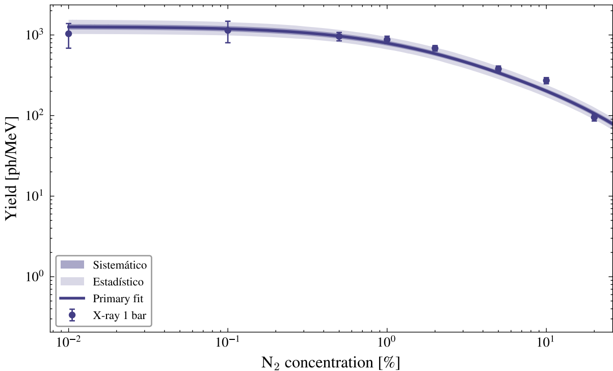
Primary Ar--N 2 IR prediction, Ar--CF 4 norm.
