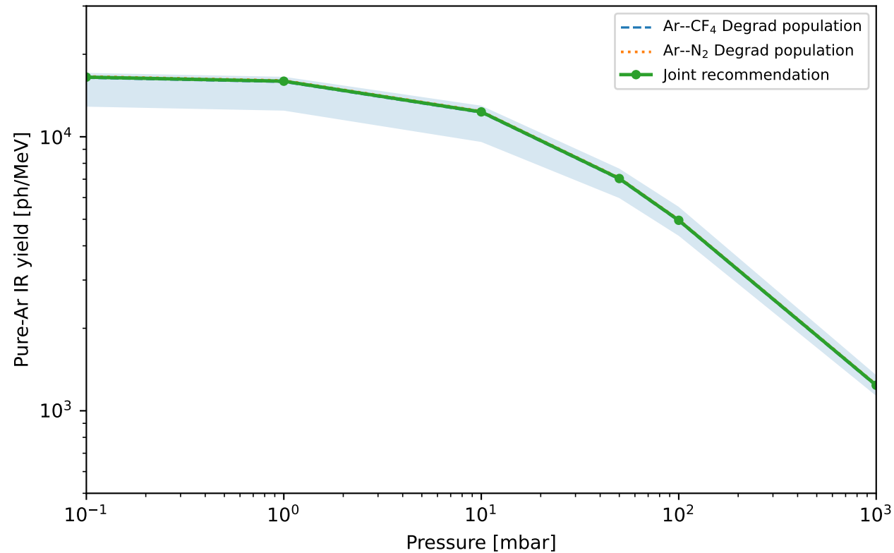
Pure-Ar IR prediction from the joint fit
