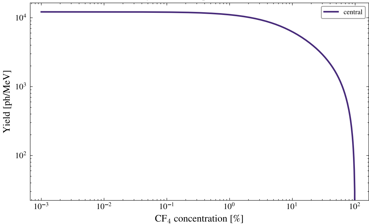
Primary Ar--CF 4 IR prediction, 10 mbar
