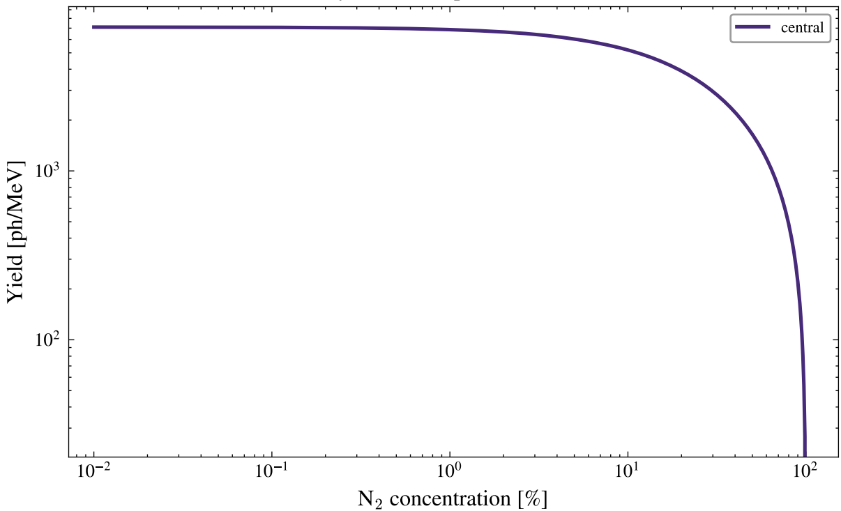
Primary Ar--N2 IR prediction, 10 mbar
