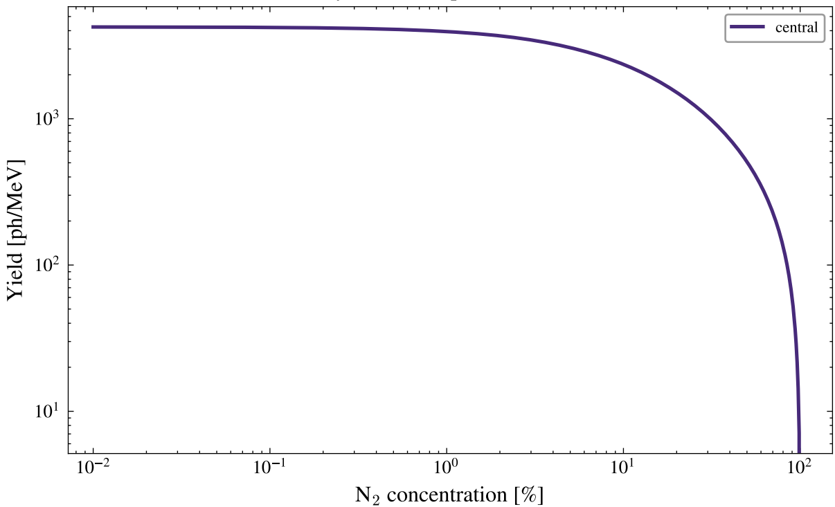
Primary Ar--N 2 IR prediction, 50 mbar
