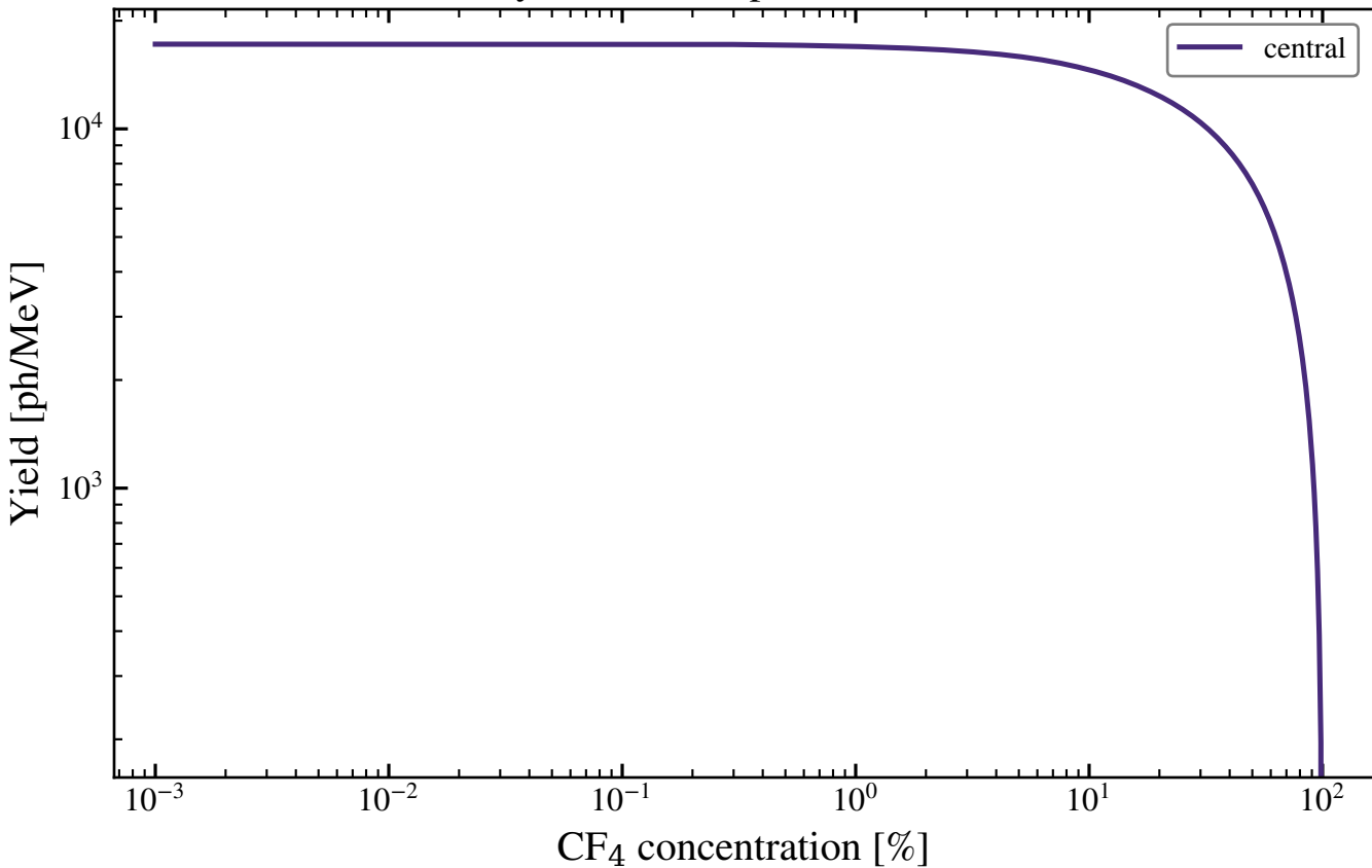
Primary Ar--CF 4 IR prediction, 0.1 mbar
