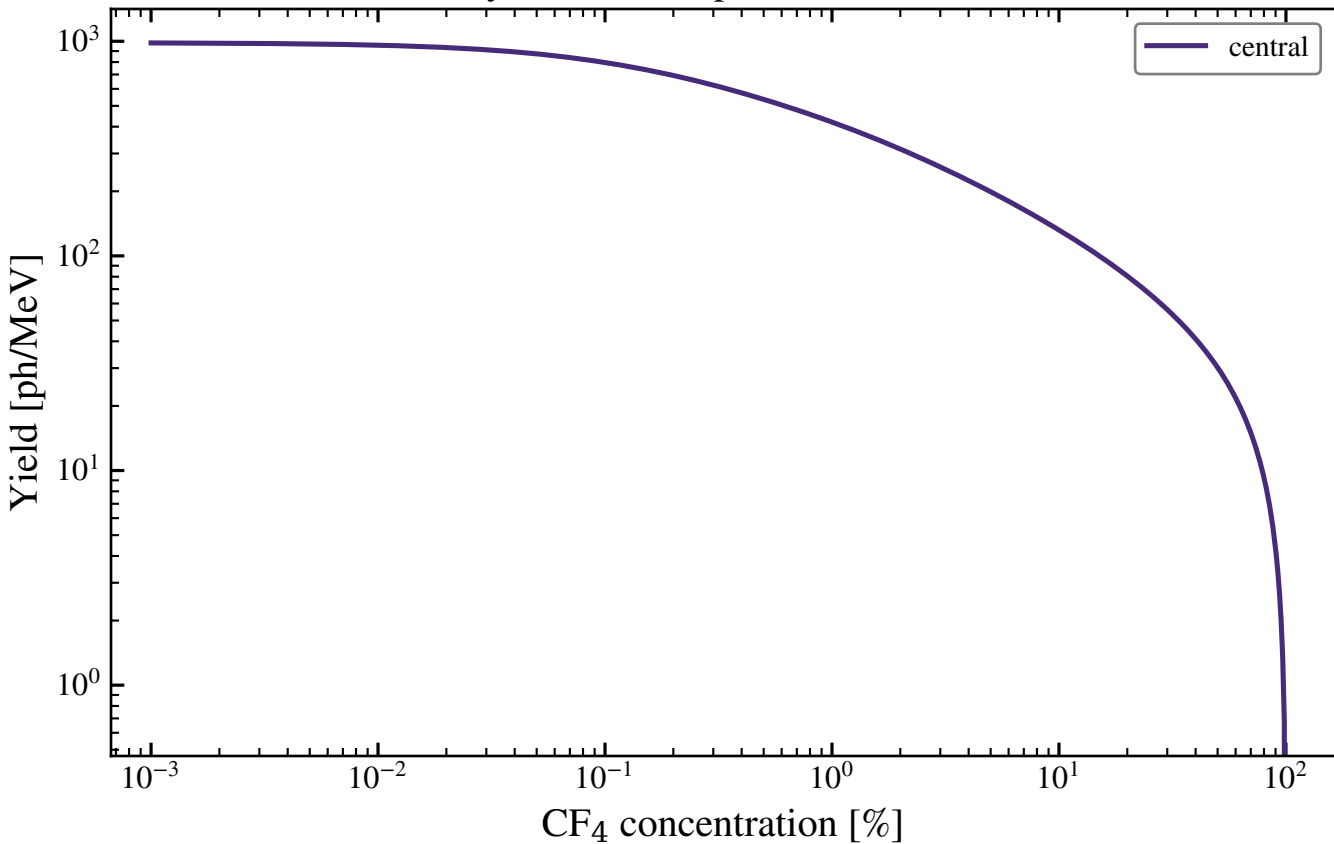
Primary Ar--CF 4 IR prediction, 1000 mbar
