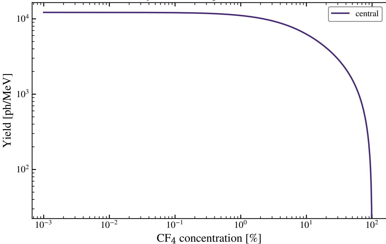
Primary Ar--CF 4 IR prediction, 10 mbar
