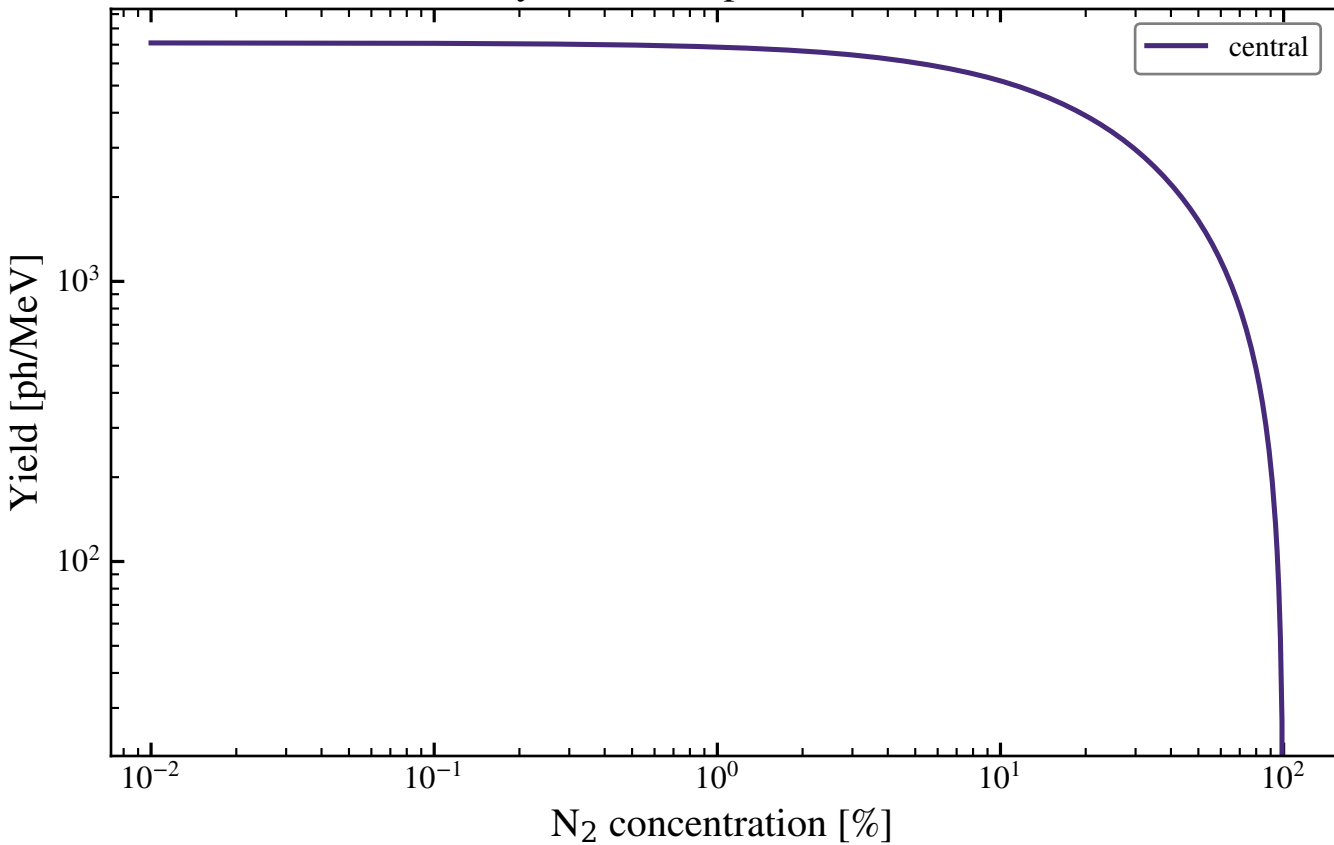
Primary Ar--N 2 IR prediction, 10 mbar
