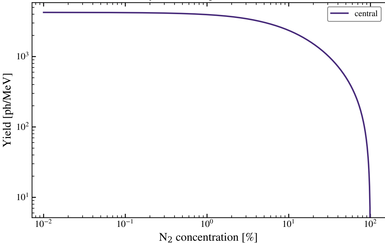
Primary Ar--N 2 IR prediction, 50 mbar
