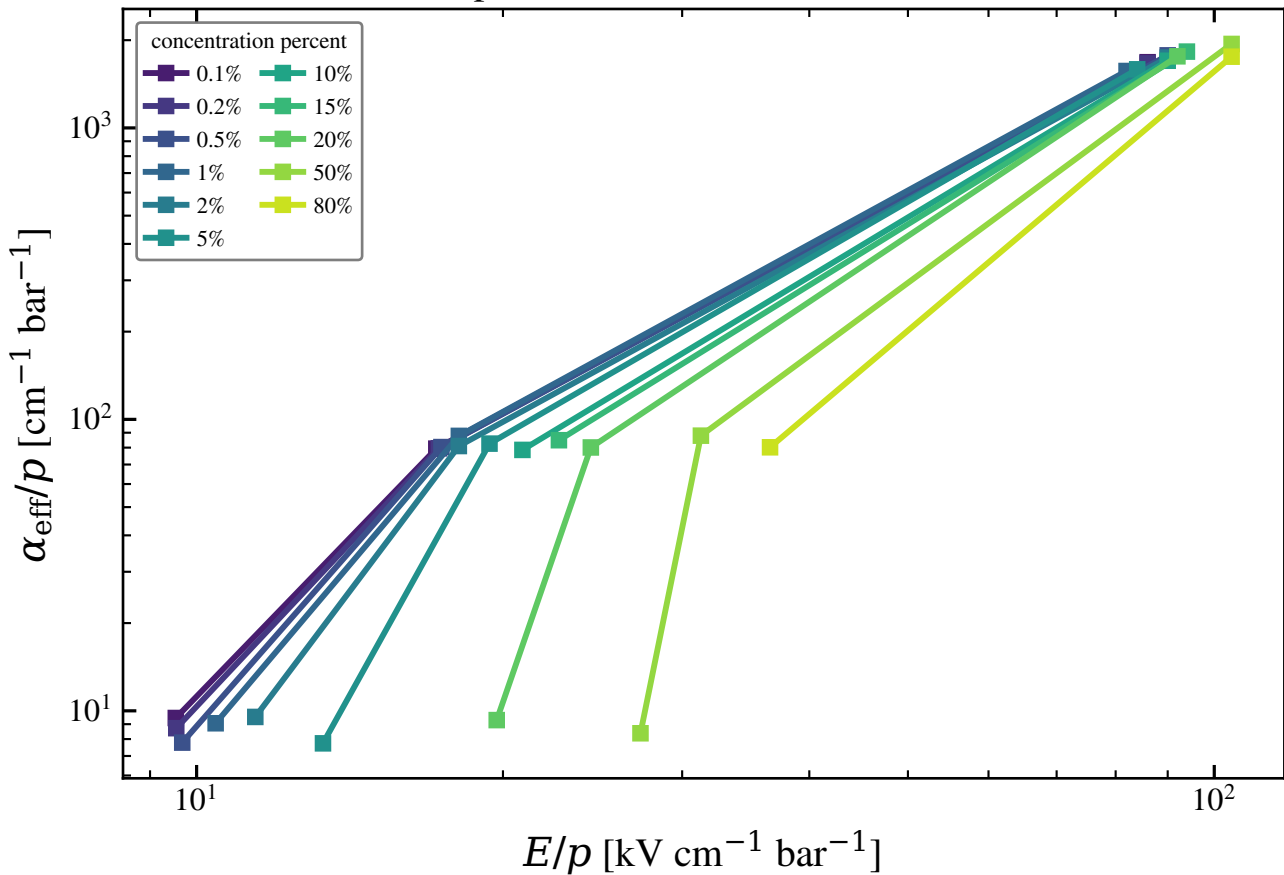
arcf4 alpha eff vs reduced field — THGEM
