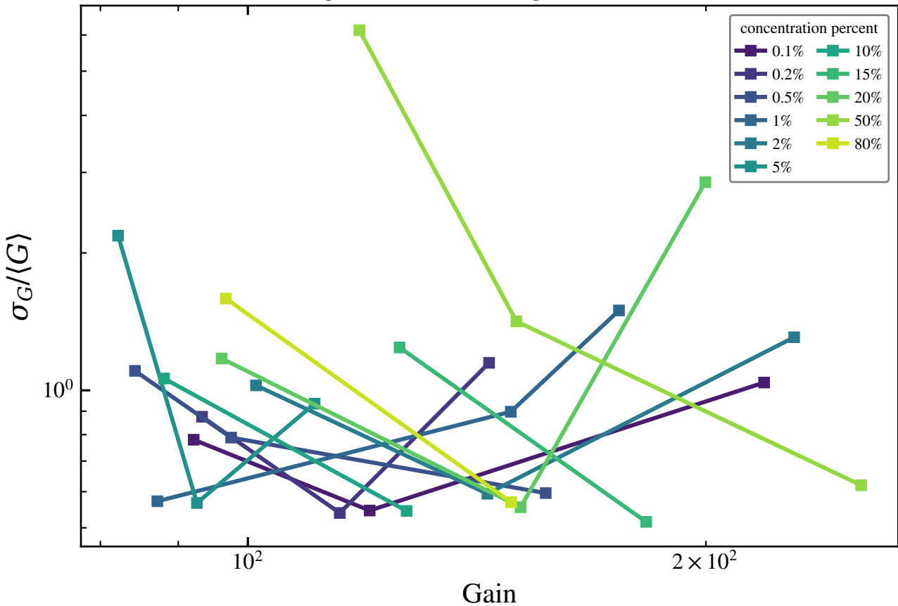
arcf4 gain resolution vs gain — THGEM
