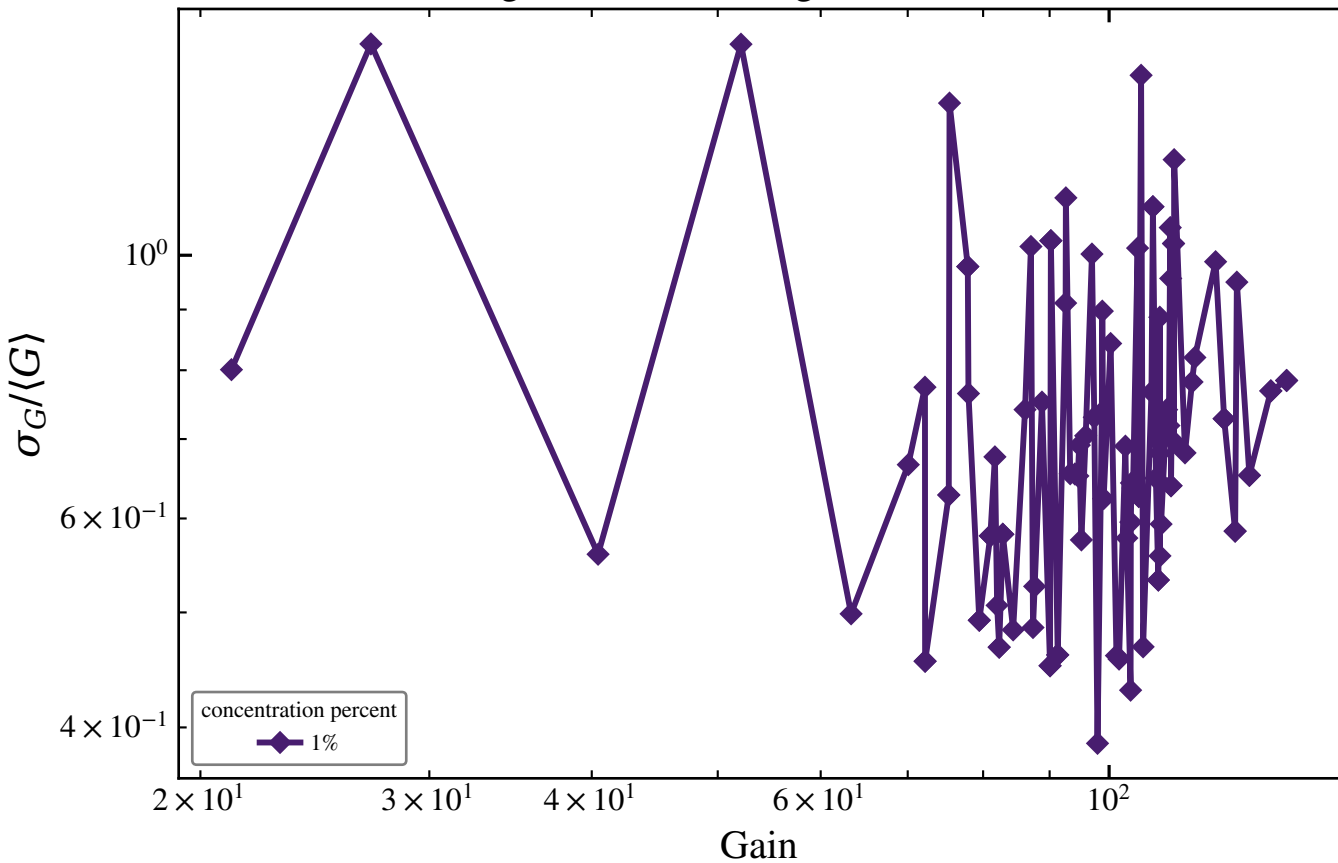
arcf4 gain resolution vs gain — UNIFORM
