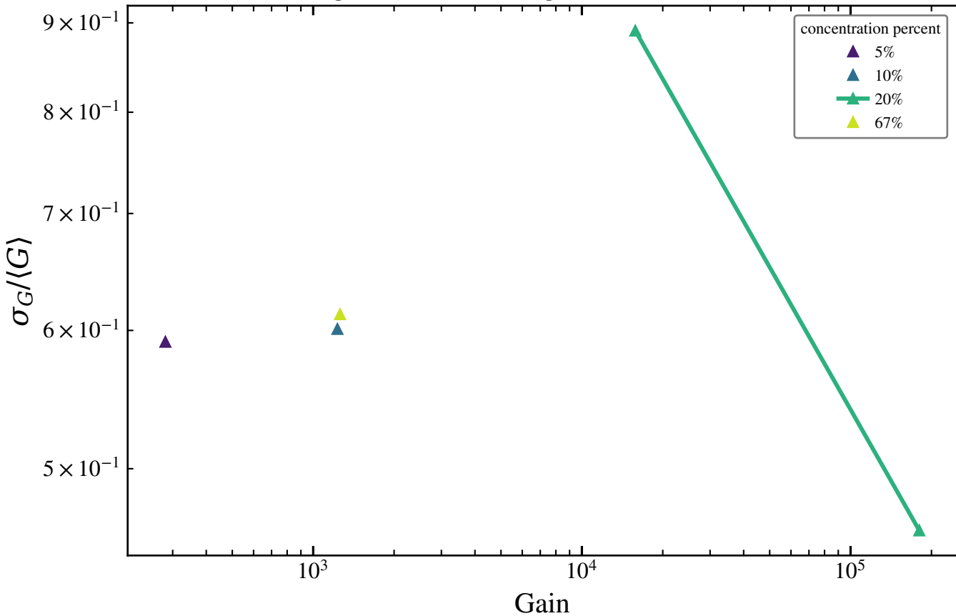
arcf4 gain resolution vs gain — UNSPECIFIED
