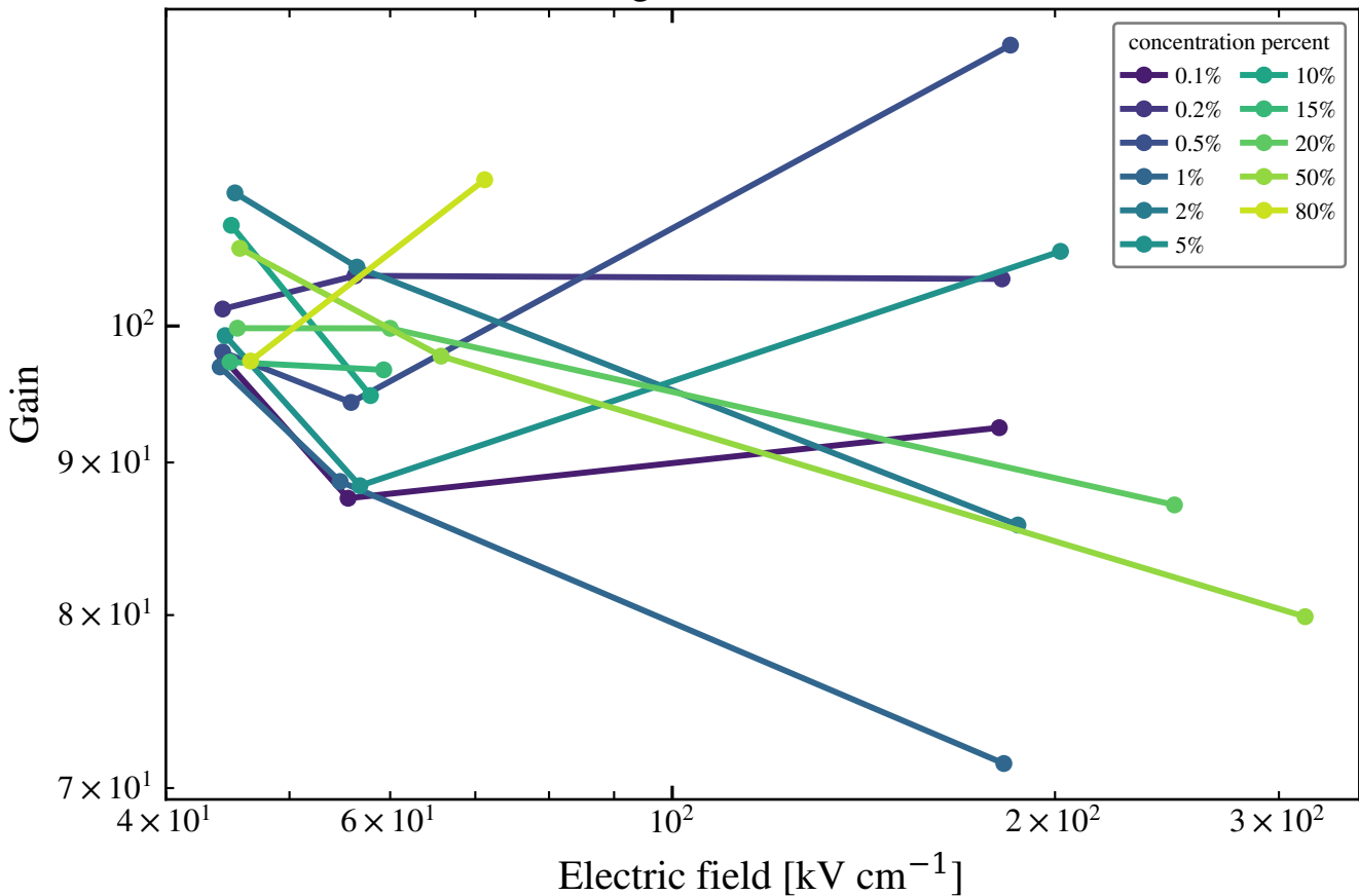
arcf4 gain vs field — GEM
