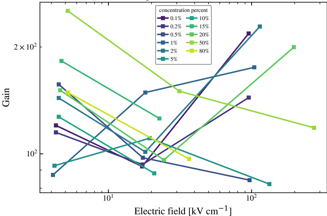
arcf4 gain vs field — THGEM
