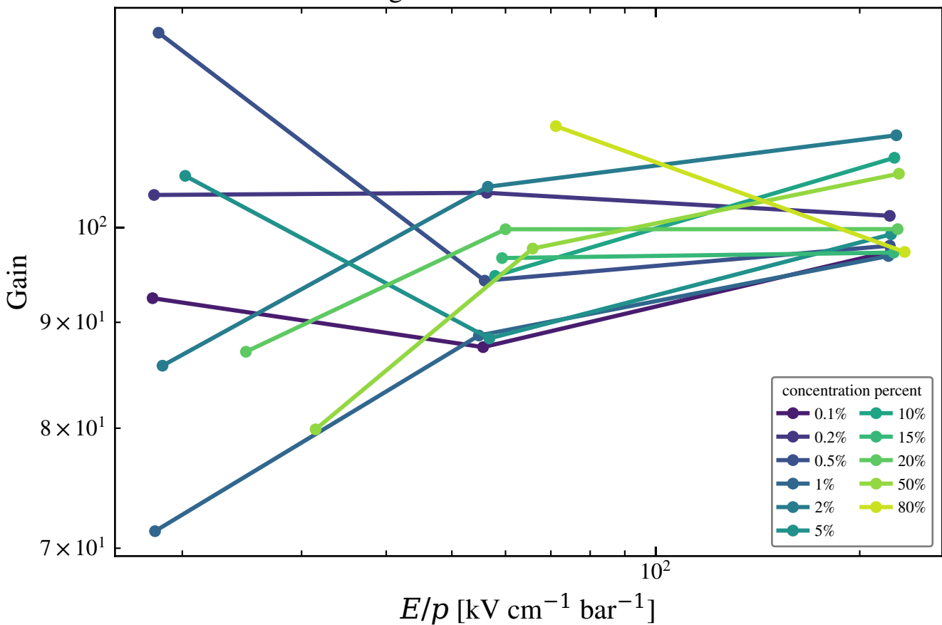
arcf4 gain vs reduced field — GEM
